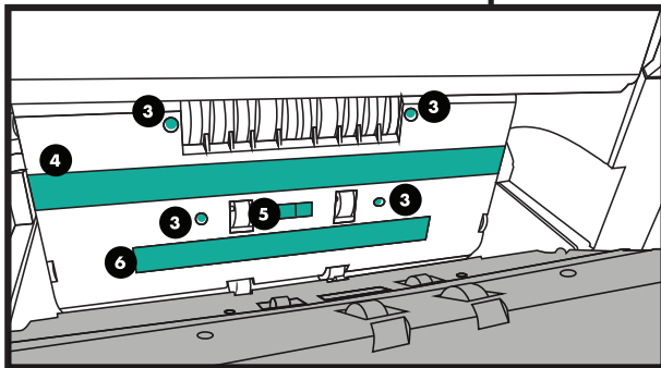
Figure 4: Inner sensors - Four pairs of positioning sensors, two large CIS sensor bars, two UV sensors, two large MG sensor bars.
